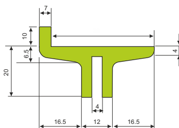
Uπ 45 LATERAL
