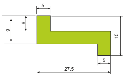
Z 27.5
